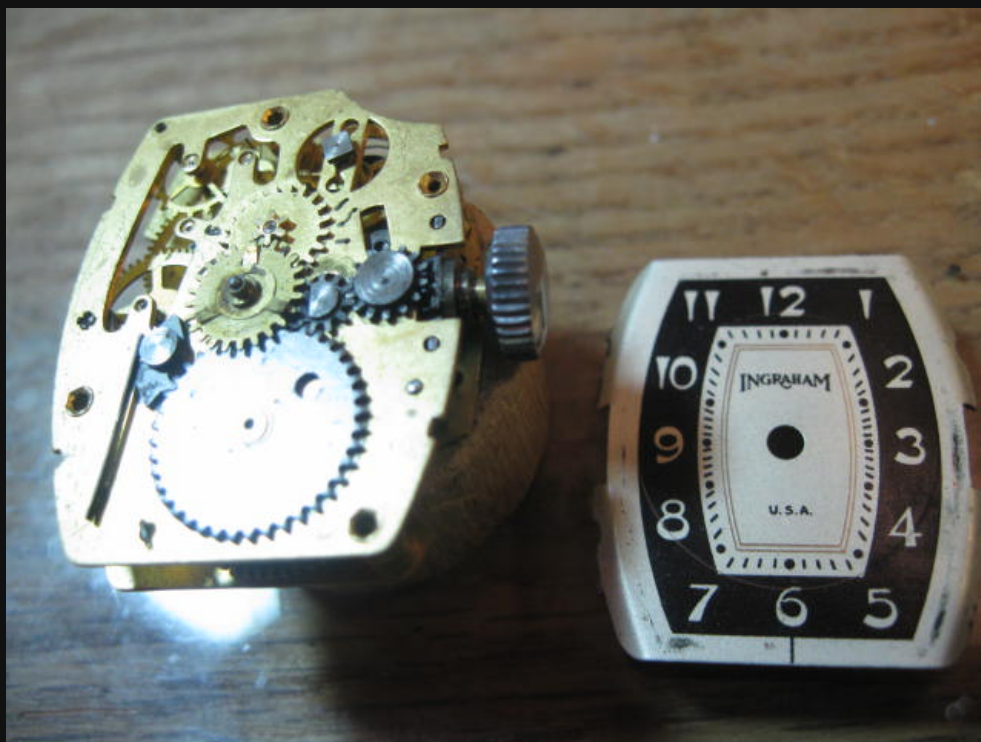
HOUR WHEEL, RATCHET WHEEL & CLICK/CLICK SPRING
