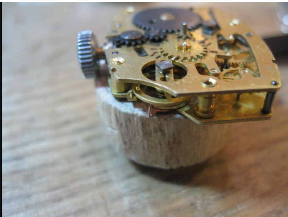
PINION GEAR INSTALLED OILED AND LUBED
